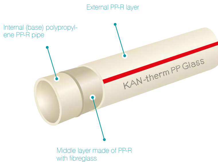
Compound pipes KAN-therm PP Glass
