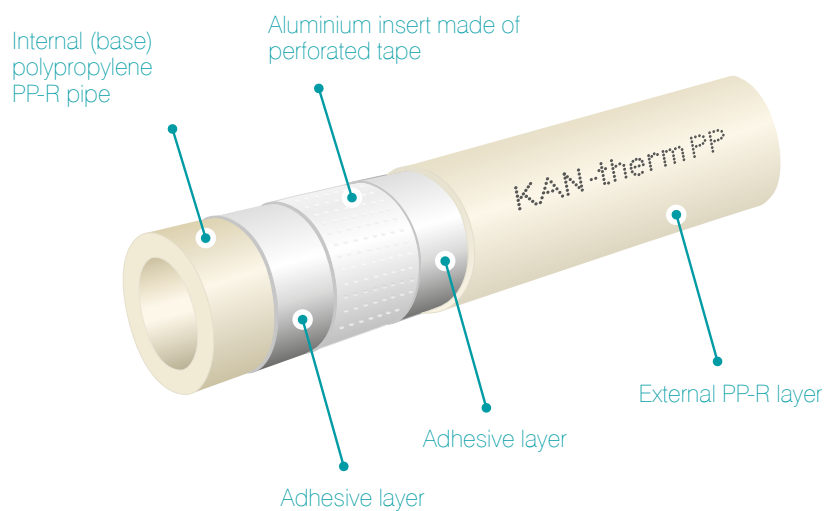
Compound pipes KAN-therm PP Stabi Al
